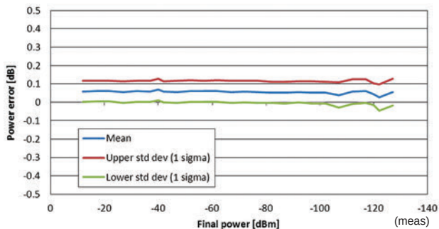
Linearity
