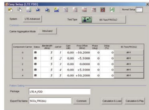
MX370108A LTE IQproducer/MX370108A-001 LTE-Advanced FDD Option LTE-Advanced Easy Setup Screen
