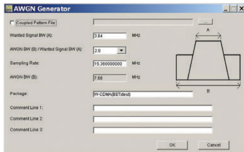
AWGN Screen
