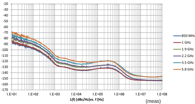
SSB Phase Noise
