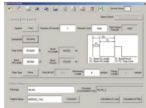
MX370111A WLAN IQproducer/MX370111A-002 802.11ac (160 MHz) Option WLAN IEEE802.11ac Easy Setup Screen
