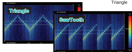
10 points, 500- \mu s Dwell Time
