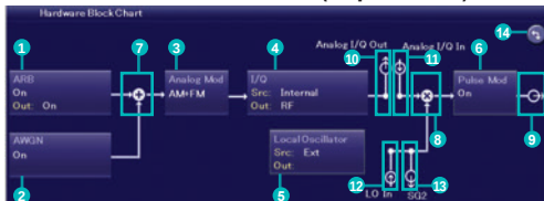
Hardware Block Chart (Explanation)
